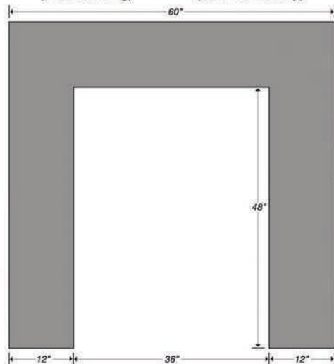
48" Indicator column (Free standing)
